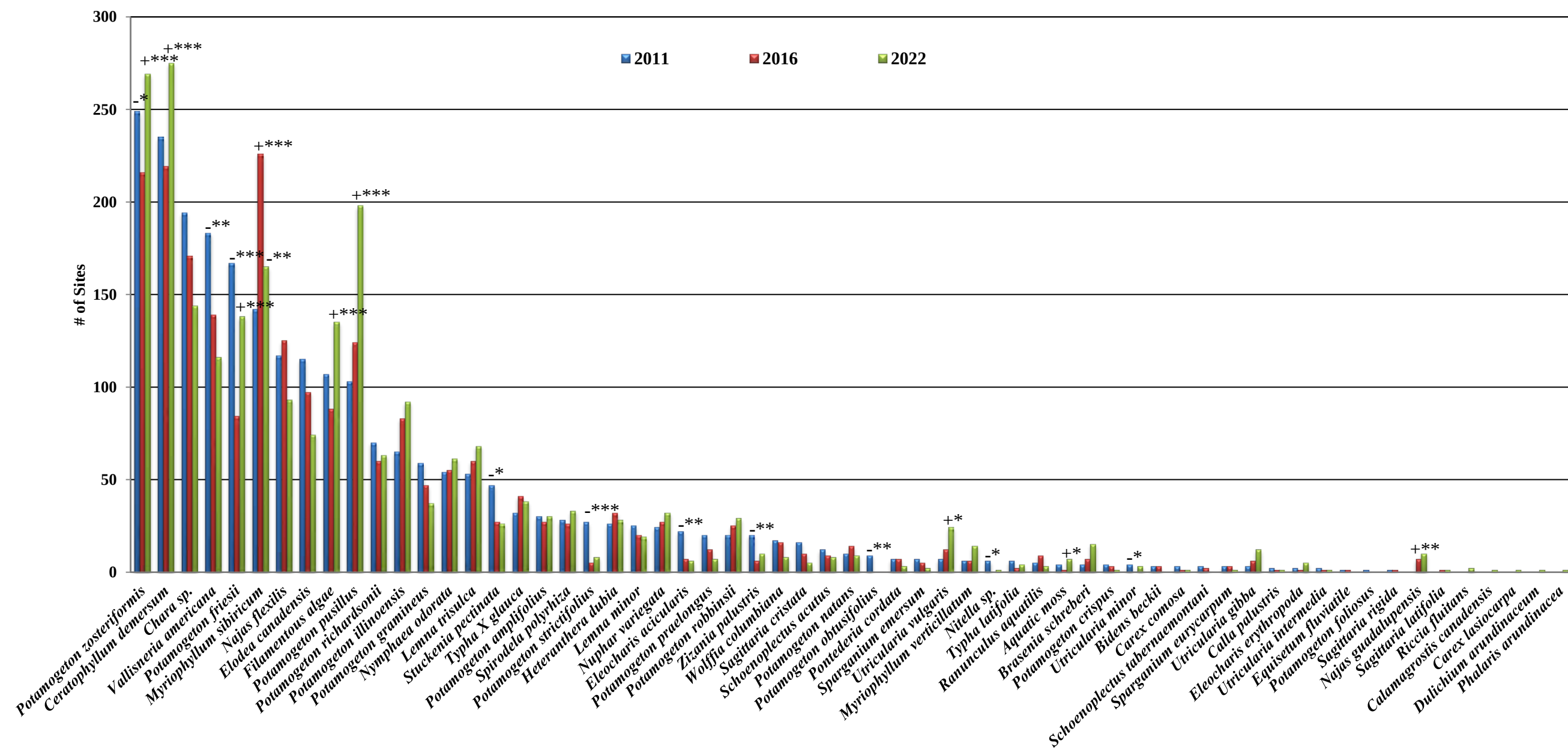
Figure 8: Macrophytes Showing Significant Changes from 2011-2016-2022
