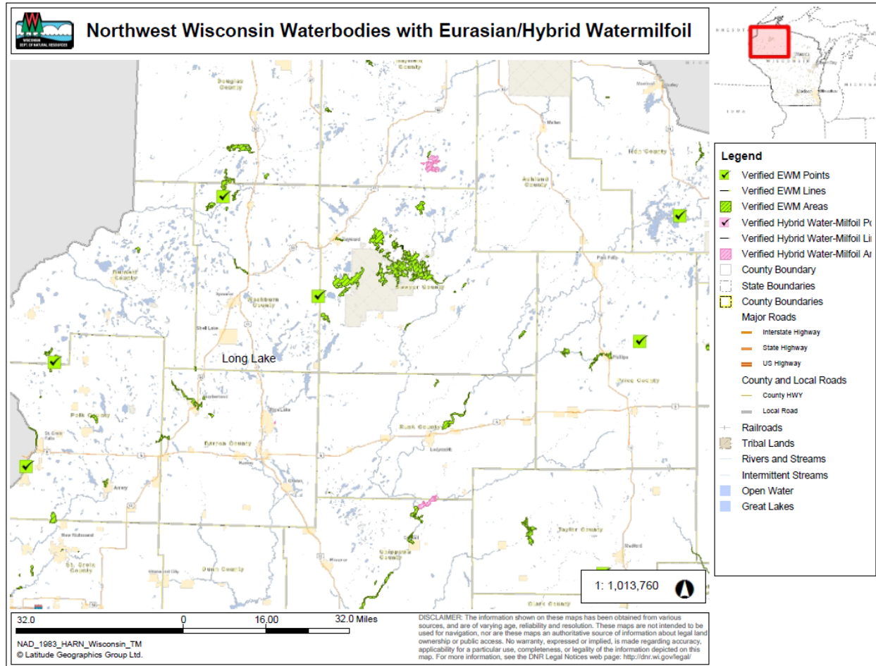
FIGURE 18. MAP OF NORTHWEST WISCONSIN VERIFIED OCCURRENCES OF EWM AND HWM
